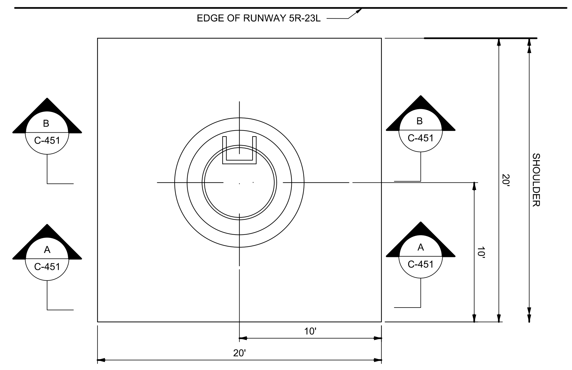
PLAN - COVER SLAB NTS
