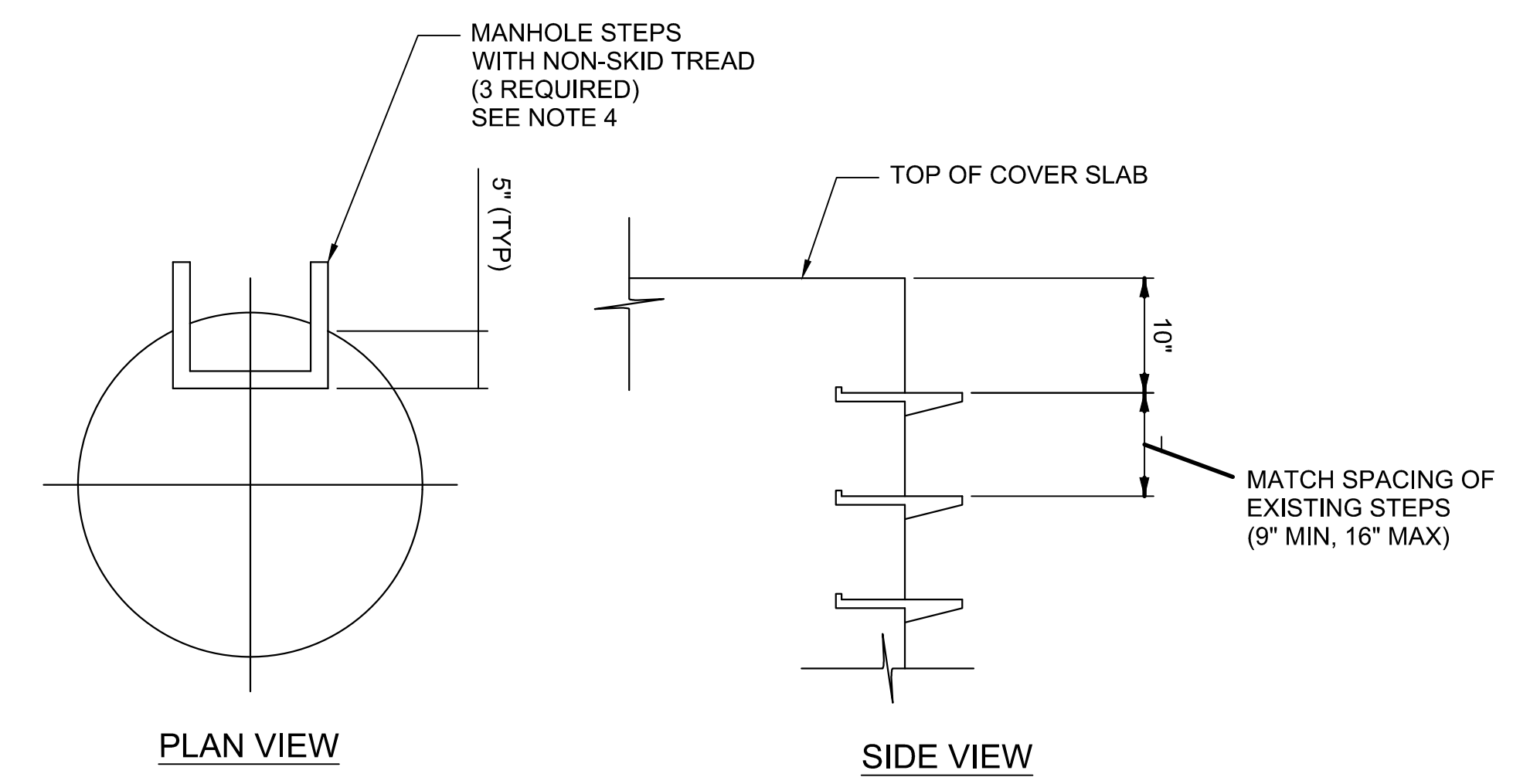
MANHOLE STEP CONFIGURATION NTS
